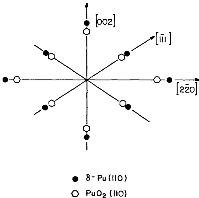
Fig. 6. Schematic (110) SAD showing indexing of diffraction spots for Pu-1.5 wt% Ga and the epitaxial PuO 2 .
